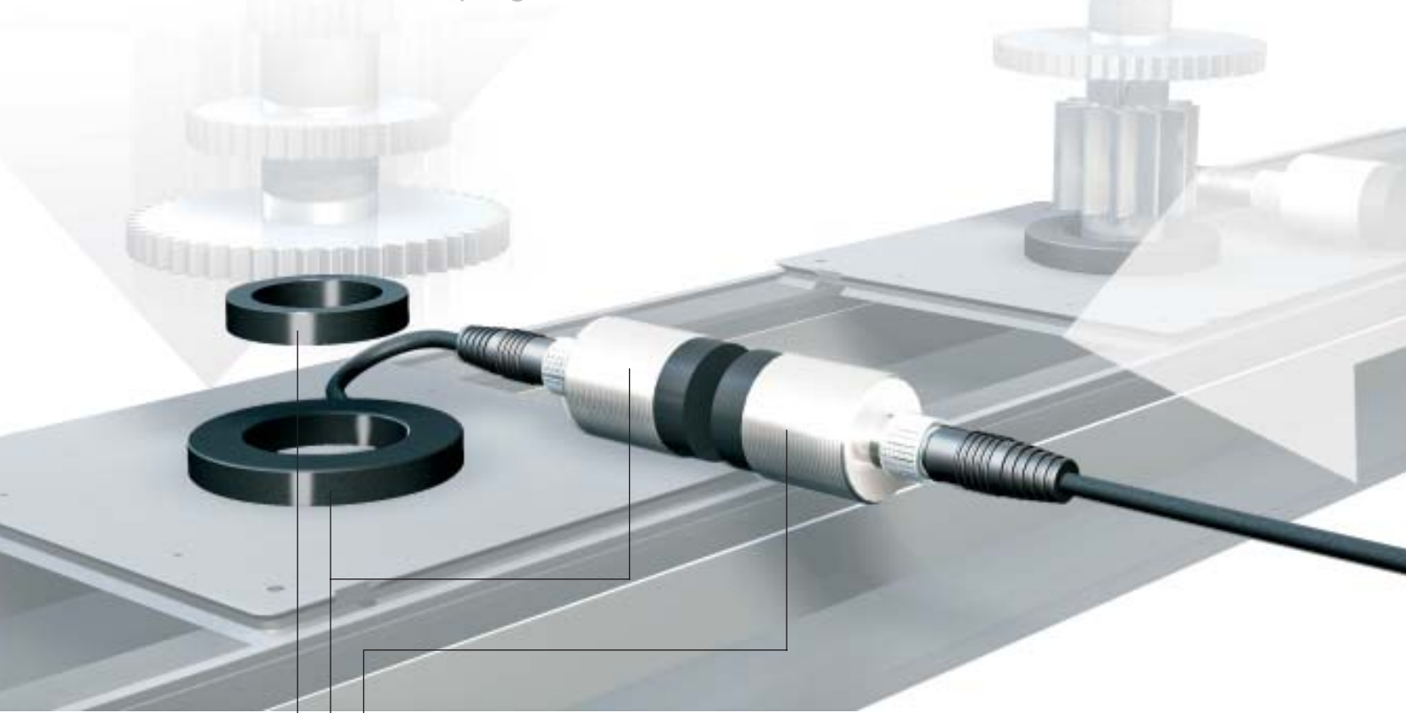
Read/write head Data coupler Data carrier
